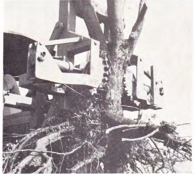
Trees easily transported whole, alternatively the tree may be felled leaving 76 cm (2' 5") of the stump for the machine to grip.
